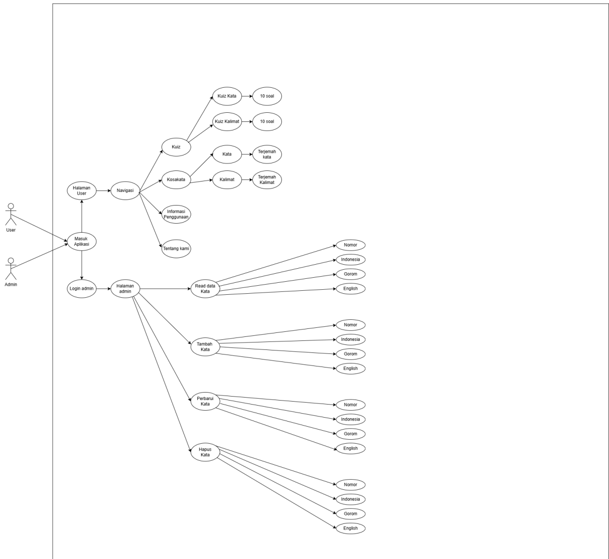
Usecase Diagram
